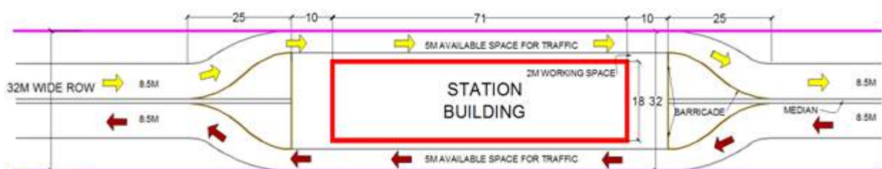
FIGURE 5.57: TYPICAL TRAFFIC DIVERSION PLAN (ROW > 32M)
