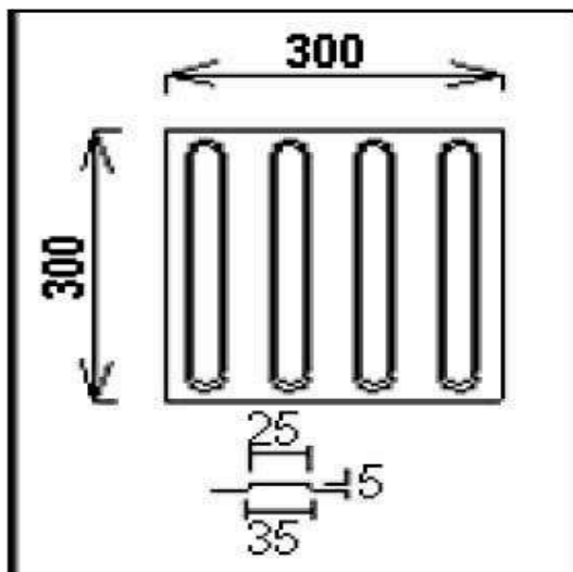
FIGURE 6.5: GUIDING PAVER
