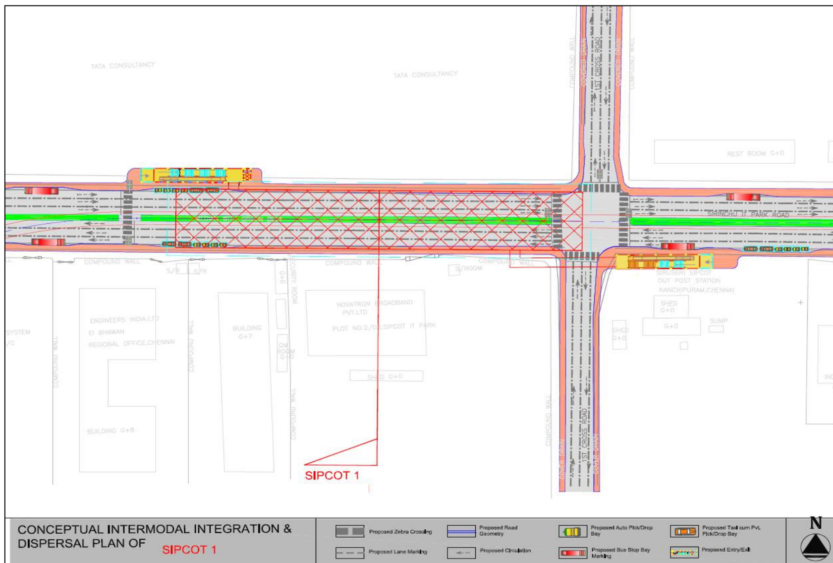
ANNEXURE 7.13. PROPOSED INTERMODAL INTEGRATION AND DISPERSAL PLAN OF SIPCOT 1 STATION
