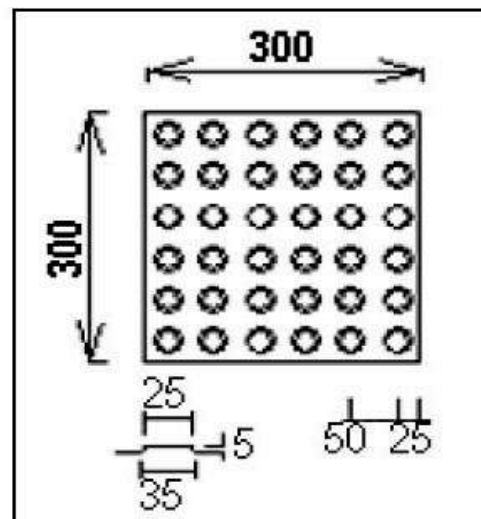
FIGURE 6.6: WARNING PAVER
