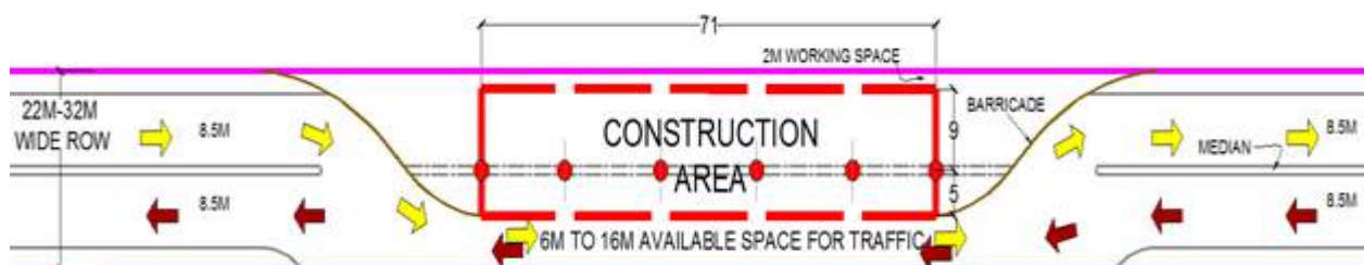
FIGURE 5.58: TYPICAL TRAFFIC DIVERSION PLAN (ROW < 32M)
