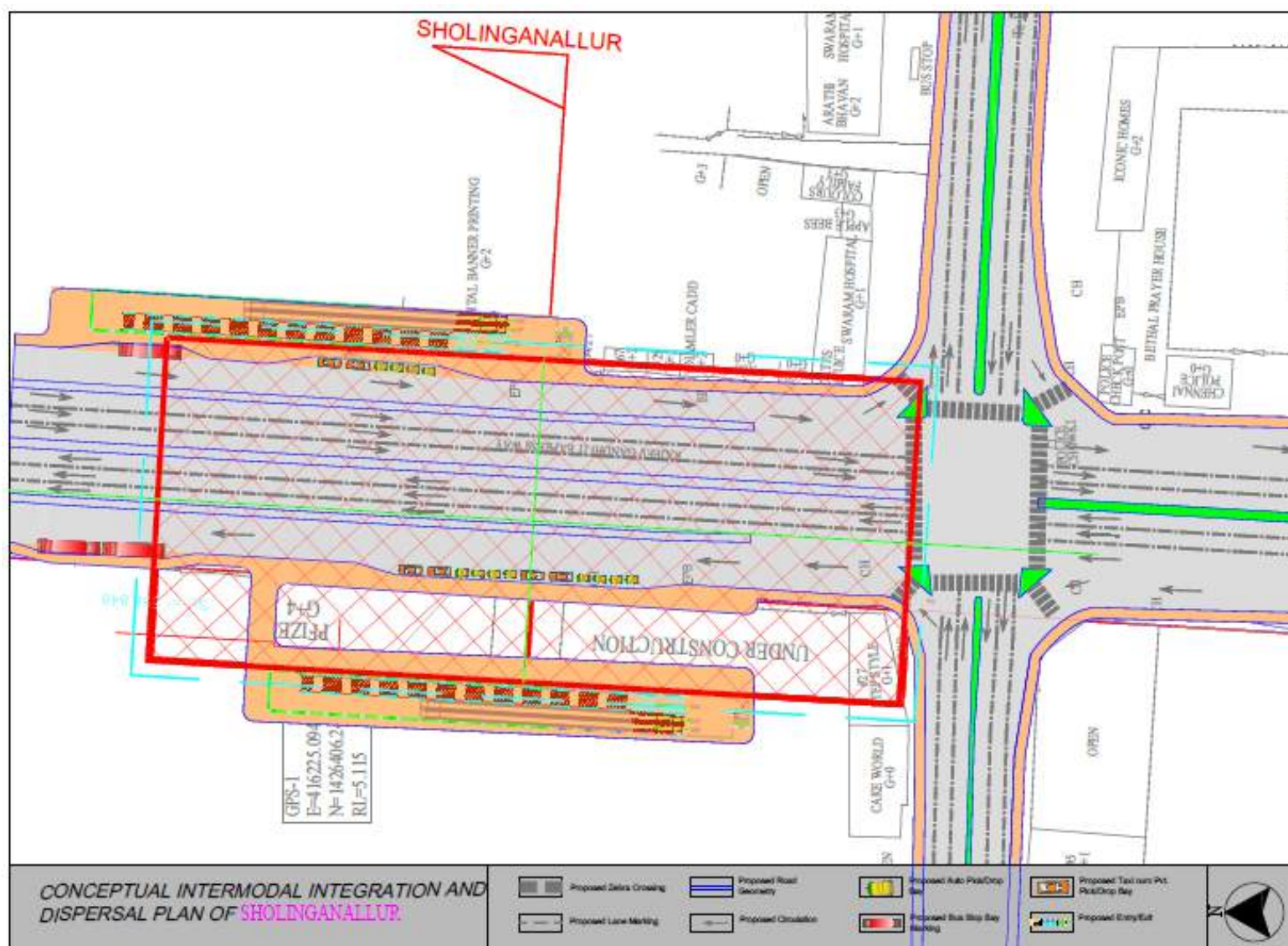
ANNEXURE 7.29. PROPOSED INTERMODAL INTEGRATION AND DISPERSAL PLAN OF SHOLINGANALLUR STATION
