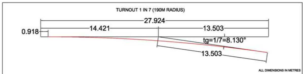
FIGURE 5.4: 1 IN 7 TYPE TURN-OUT (190M LEAD RADIUS)
