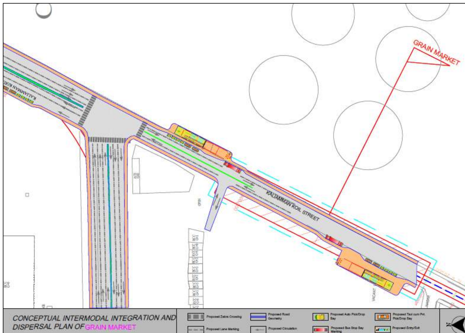
ANNEXURE 7.23. PROPOSED INTERMODAL INTEGRATION AND DISPERSAL PLAN OF GRAIN MARKET STATION
