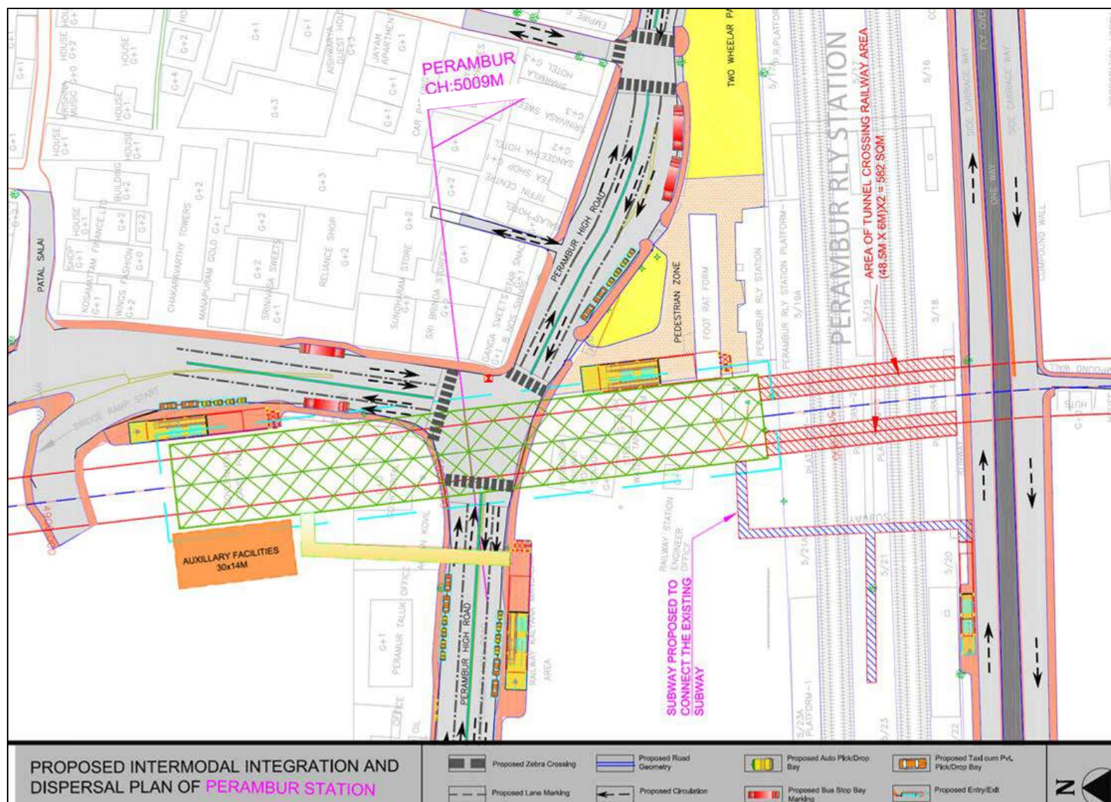
ANNEXURE 7.1. PROPOSED INTERMODAL INTEGRATION AND DISPERSAL PLAN OF PERAMBUR STATION STATION
