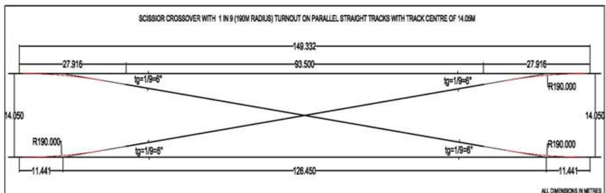
FIGURE 5.5: SCISSOR CROSS-OVER WITH 1 IN 9 TYPE TURN-OUT (190M LEAD RADIUS) ON MAIN LINES OF UNDERGROUND SECTION WITH 14.05 TRACK CENTRE
