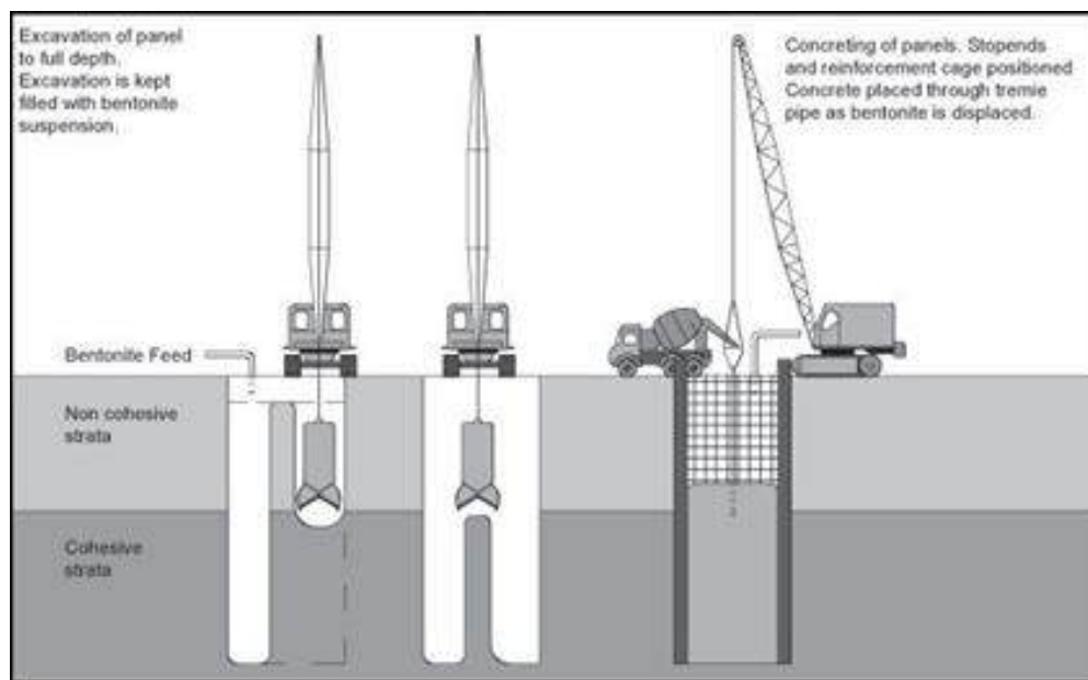
FIGURE 5.55: DIAPHRAGM WALL
