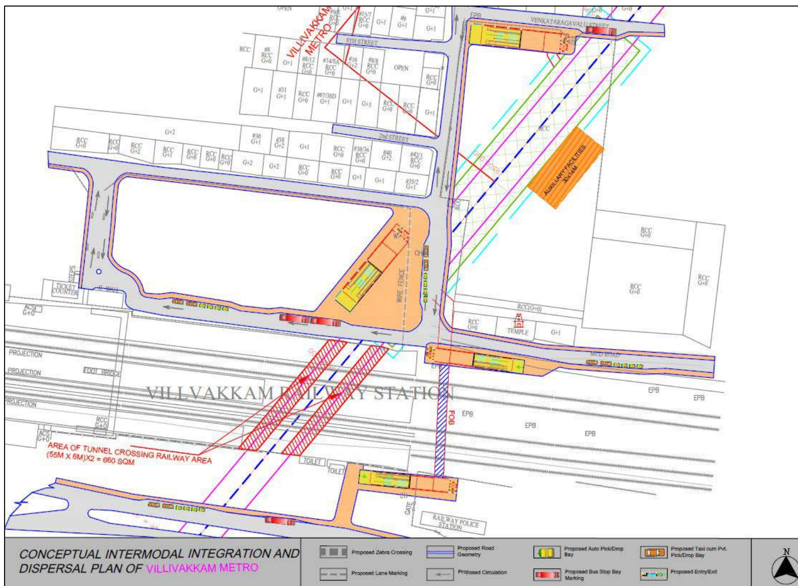
ANNEXURE 7.20. ROPOSED INTERMODAL INTEGRATION AND DISPERSAL PLAN OF VILLIVAKKAM METRO STATION
