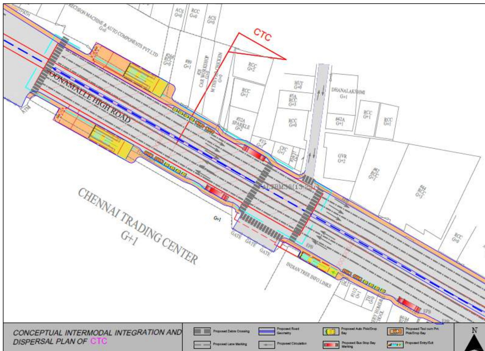
ANNEXURE 7.24. PROPOSED INTERMODAL INTEGRATION AND DISPERSAL PLAN OF CTC STATION
