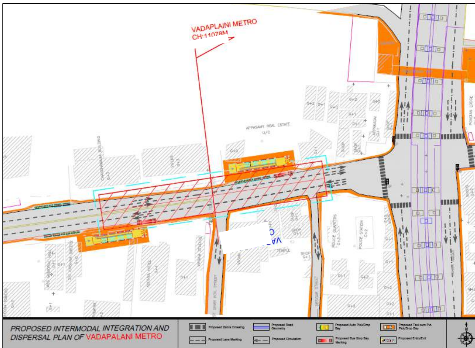
ANNEXURE 7.16. PROPOSED INTERMODAL INTEGRATION AND DISPERSAL PLAN OF VADAPALANI METRO STATION
