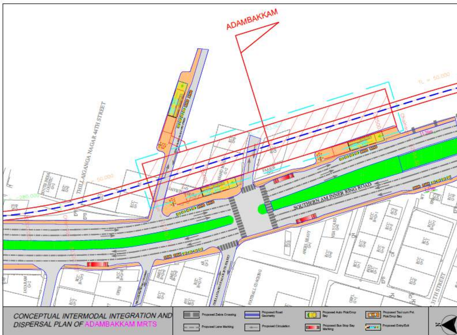
ANNEXURE 7.27. PROPOSED INTERMODAL INTEGRATION AND DISPERSAL PLAN OF ADAMBAKKAM MRTS STATION
