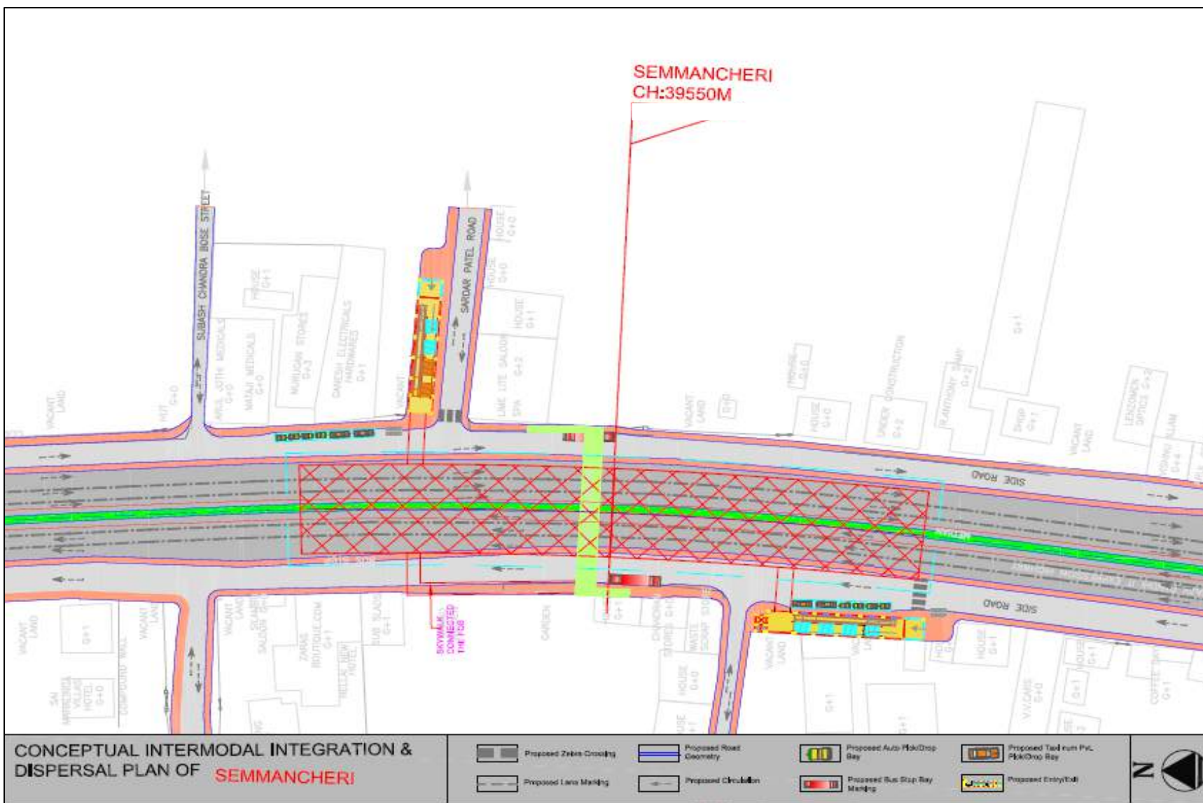
ANNEXURE 7.9. PROPOSED INTERMODAL INTEGRATION AND DISPERSAL PLAN OF SEMMANCHERI STATION
