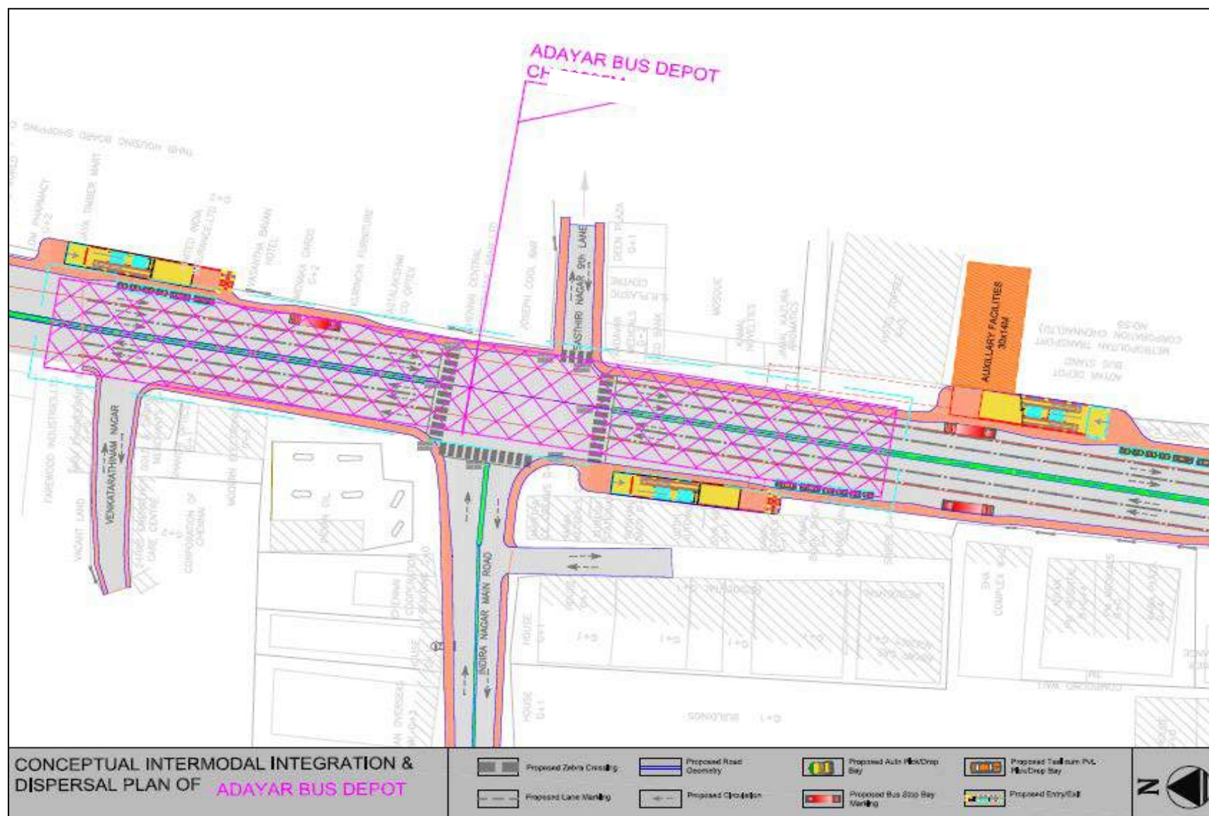
ANNEXURE 7.4. PROPOSED INTERMODAL INTEGRATION AND DISPERSAL PLAN OF ADAYAR BUS DEPOT STATION
