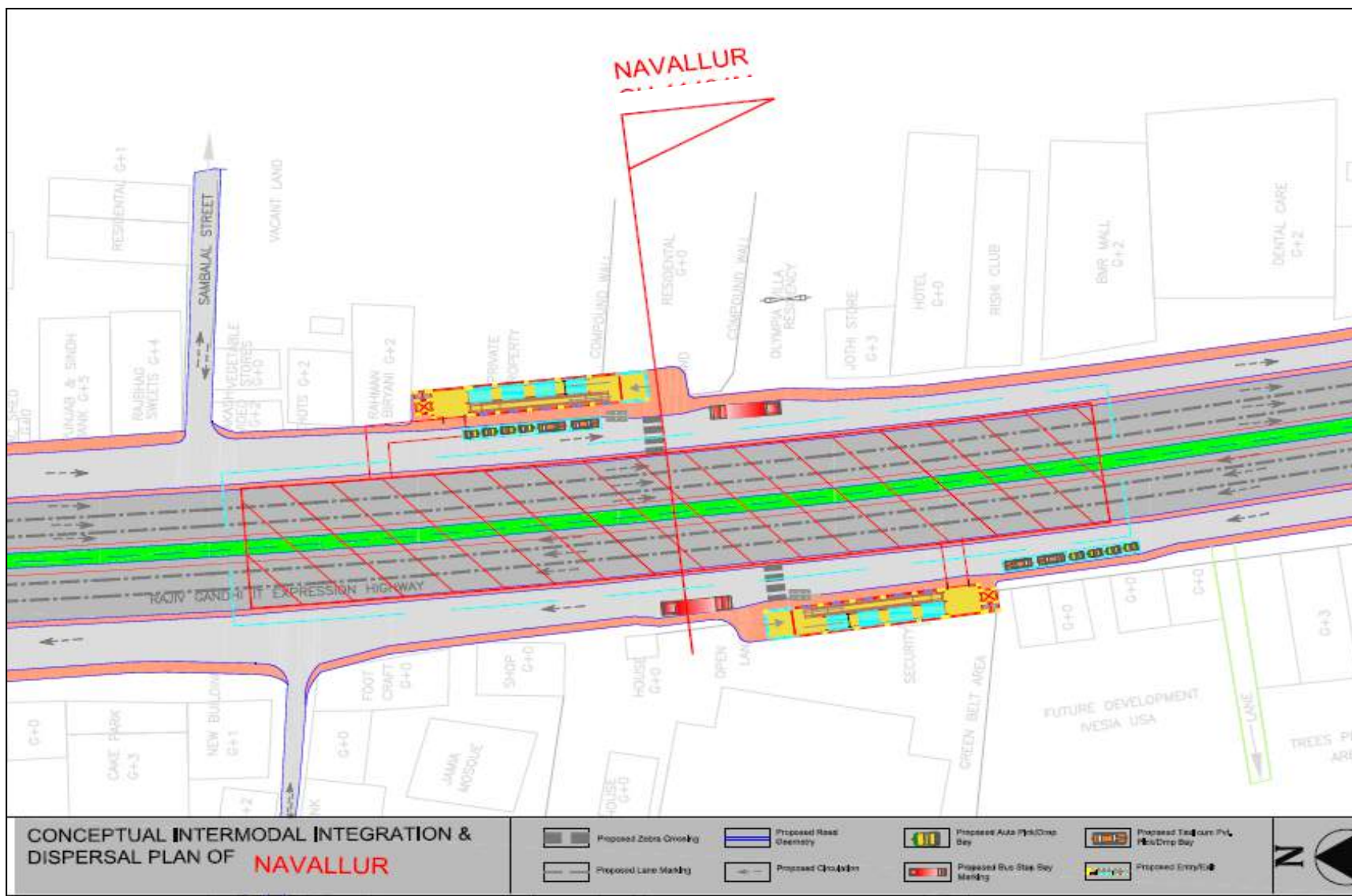
ANNEXURE 7.11. PROPOSED INTERMODAL INTEGRATION AND DISPERSAL PLAN OF NAVALLUR STATION
