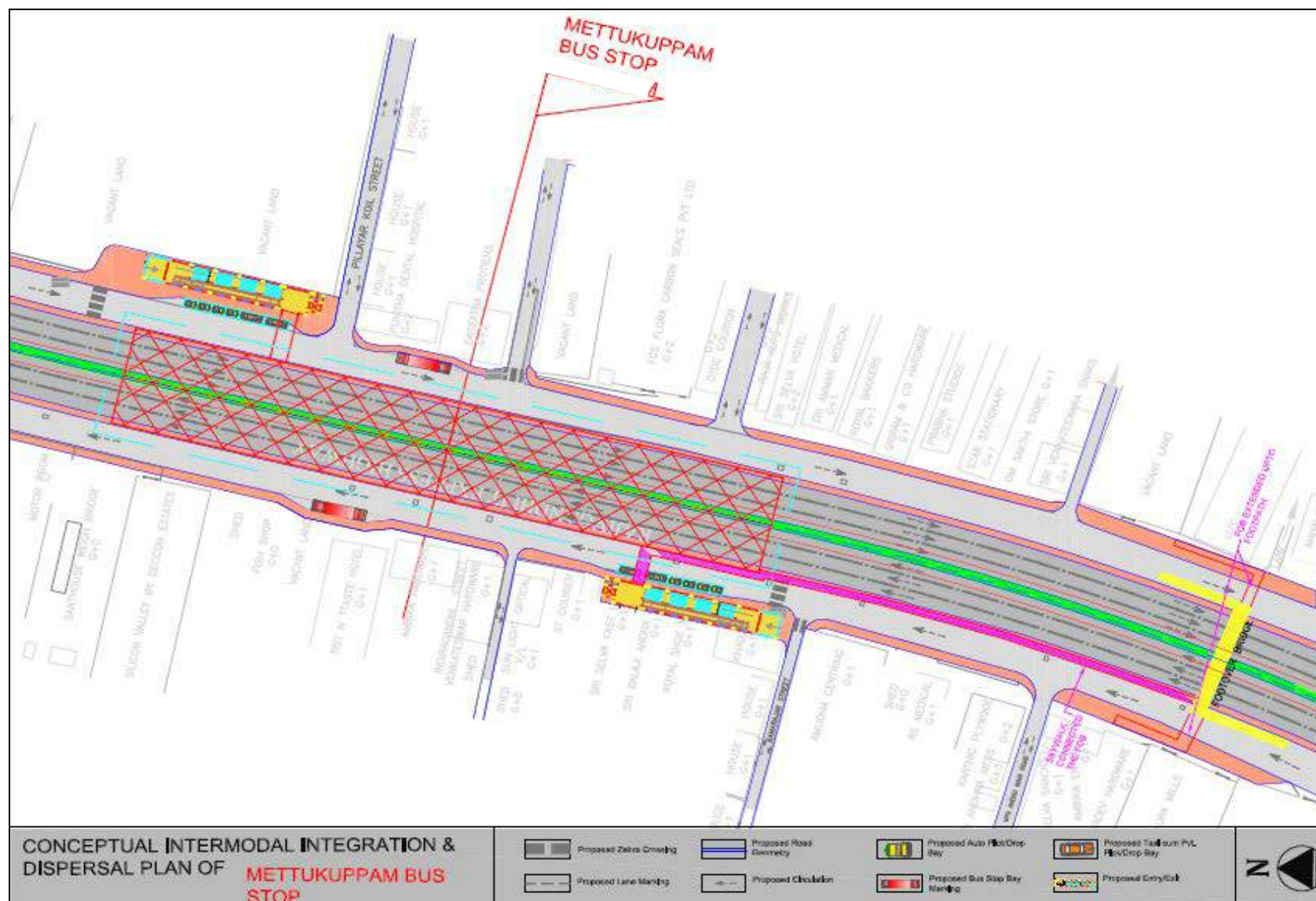
ANNEXURE 7.7. PROPOSED INTERMODAL INTEGRATION AND DISPERSAL PLAN OF METTUKUPPAM BUS STOP STATION
