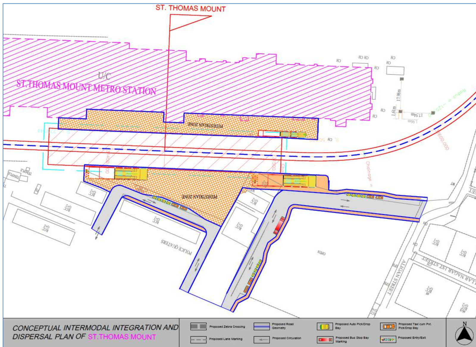
ANNEXURE 7.26. PROPOSED INTERMODAL INTEGRATION AND DISPERSAL PLAN OF ST.THOMAS MOUNT STATION
